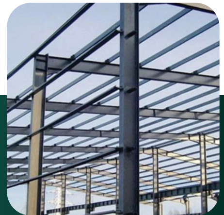
PEB Structure
